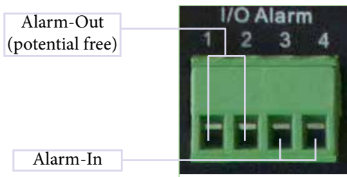
Abb. 2 Rear view
