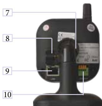
Abb. 2 Rear view
